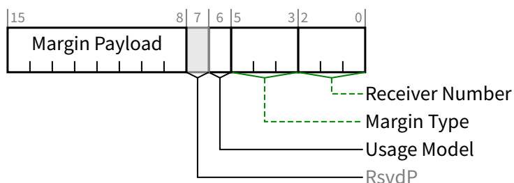
Figure 7-101 Lane N: Margining Control Register Entry
