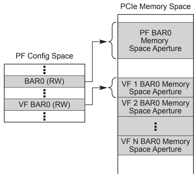
Figure 9-10 BAR Space Example for Single BAR Device
