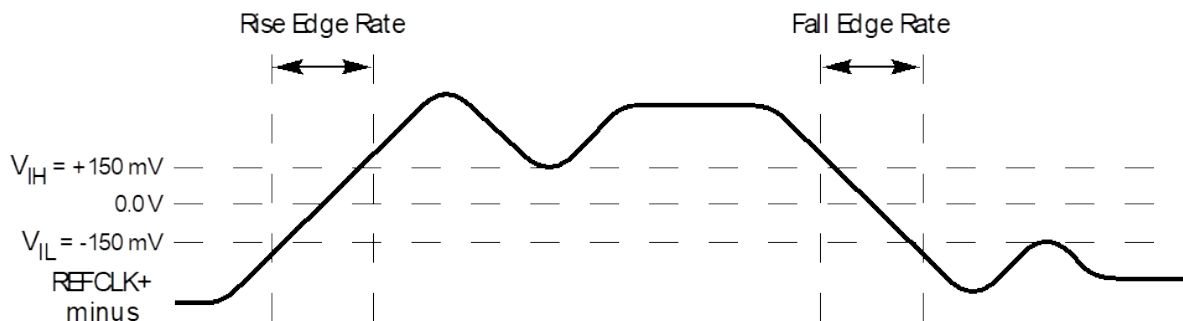
Figure 8-69 Differential Measurement Points for Rise and Fall Time
