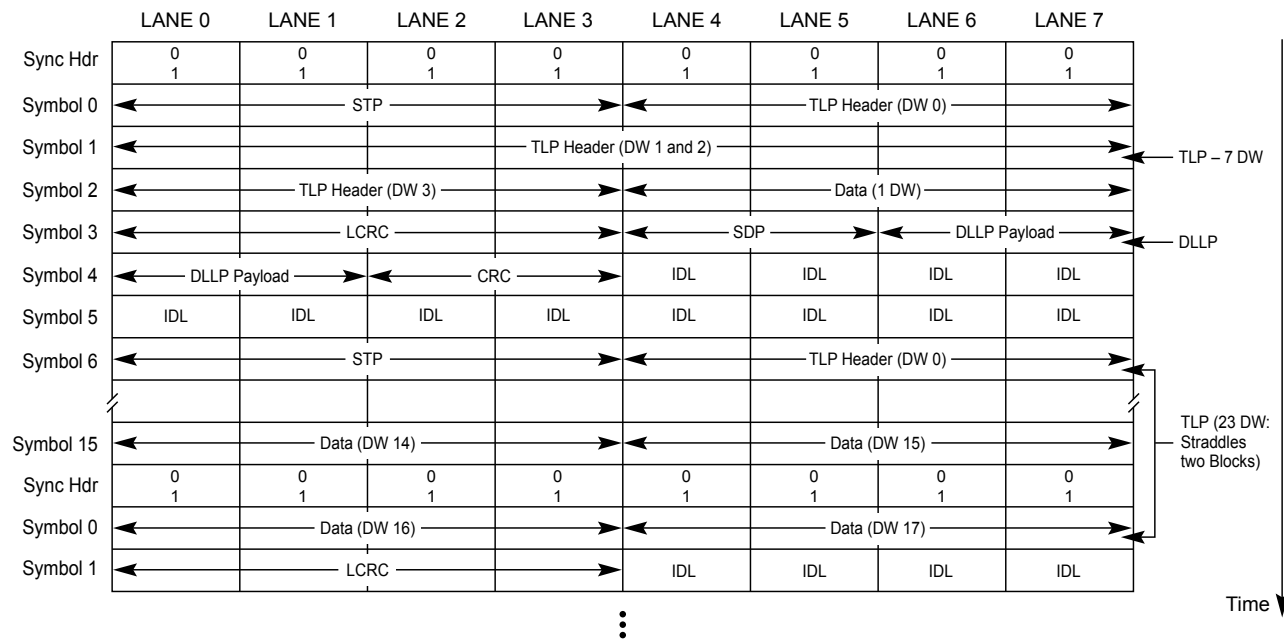
Figure 4-15 Packet Transmission in a x8 Link
