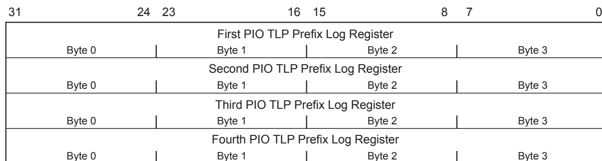
RP-PIO-TLP-Prefix-Log
