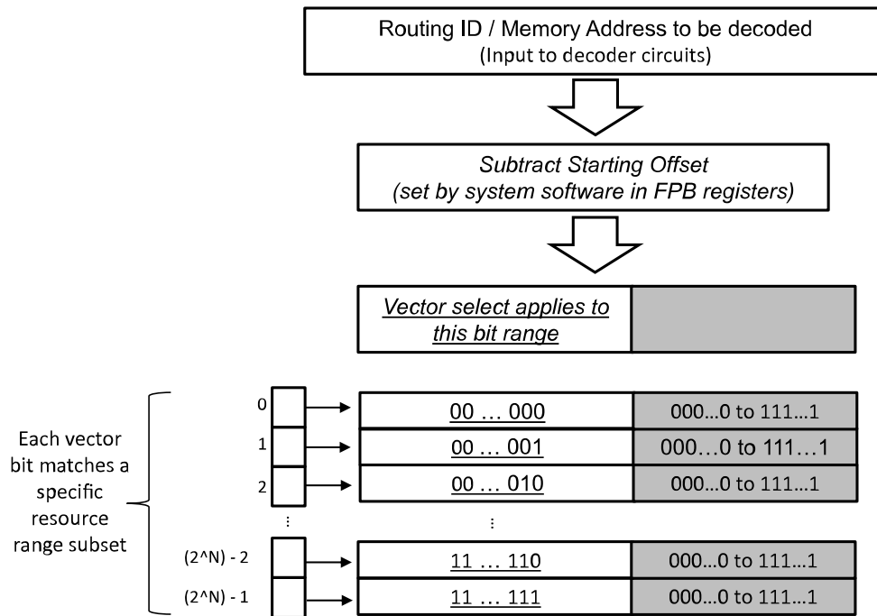
Figure 6-32 Vector Mechanism for Address Range Decoding
