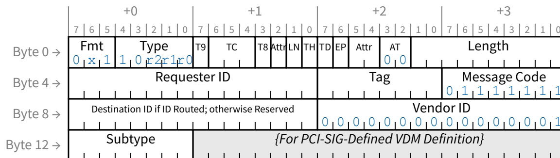
Figure 2-29 Header for PCI-SIG-Defined VDMs
