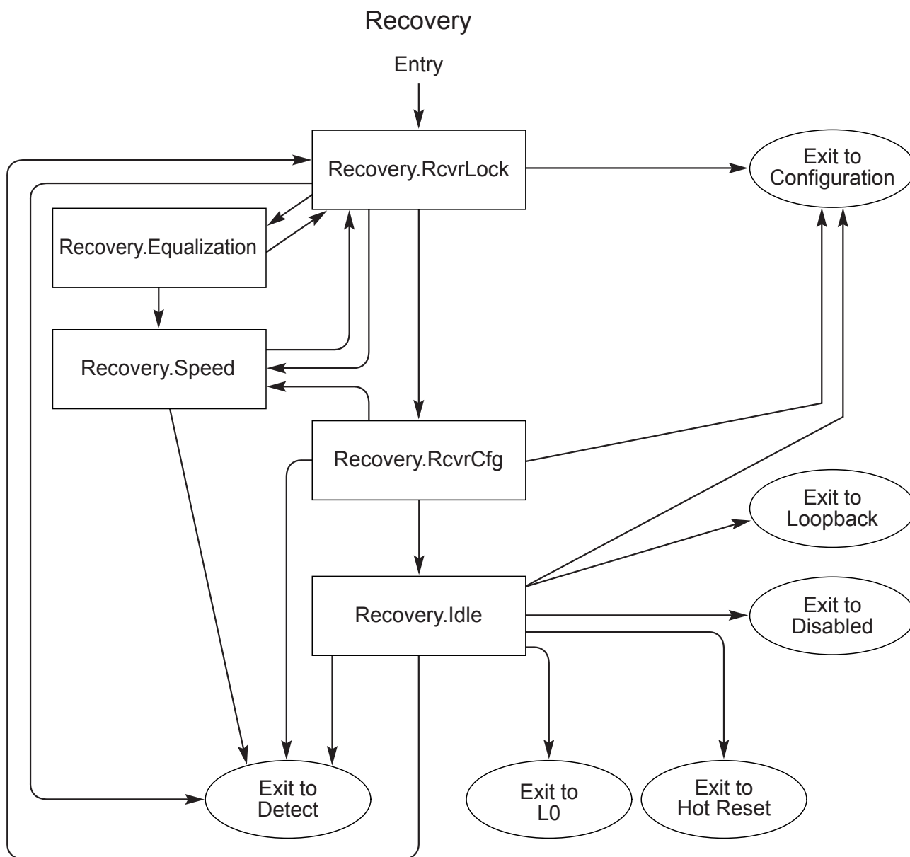
Figure 4-30 Recovery Substate Machine
