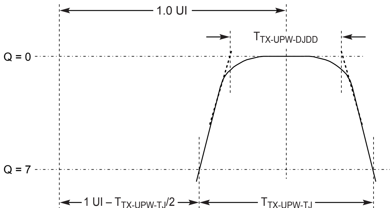
Figure 8-19 Definition of T_{TX-UPW-DJDD} and T_{TX-UPW-TJ} Data Rate Dependent Transmitter Parameters
