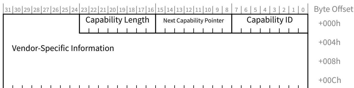
Figure 7-194 Vendor-Specific Capability
