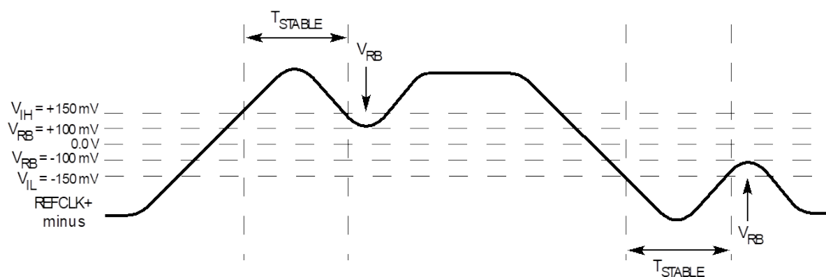
Figure 8-70 Differential Measurement Points for Ringback
