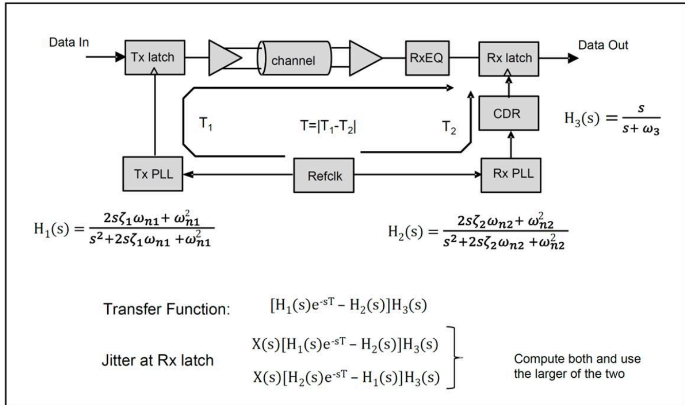
Figure 8-73 Common Refclk Rx Architecture for all Data Rates Except 32.0 GT/s
