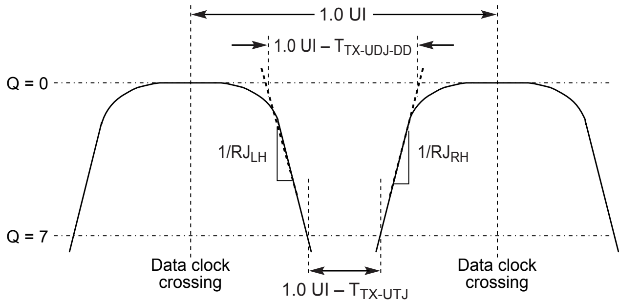
Figure 8-17 Derivation of T_{\text{TX-UTJ}} and T_{\text{TX-UDJDD}}
