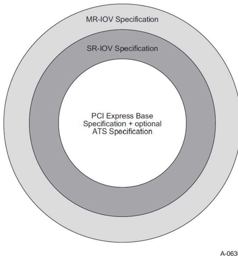
Figure 9-9 I/O Virtualization Interoperability
