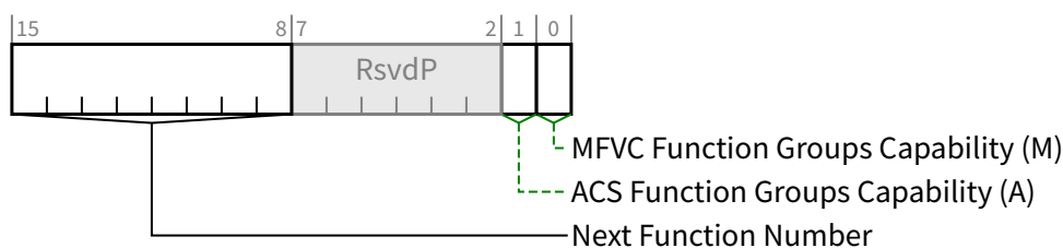
Figure 7-149 ARI Capability Register
