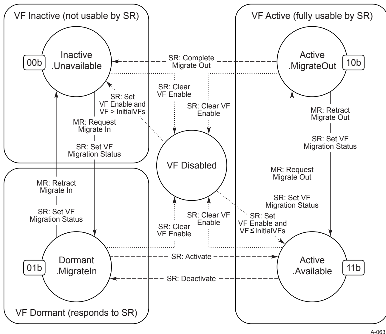
Figure 9-12 VF Migration State Diagram
