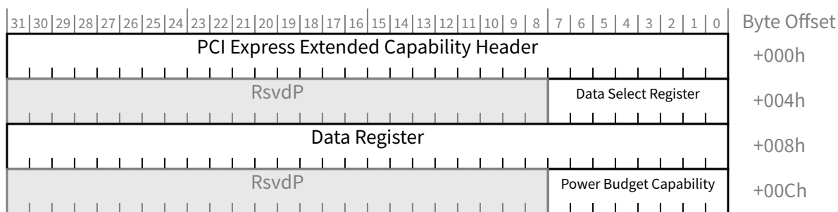
Figure 7-108 Power Budgeting Extended Capability
