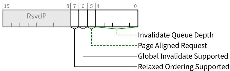
Figure 10-21 ATS Capability Register (Offset 04h)
