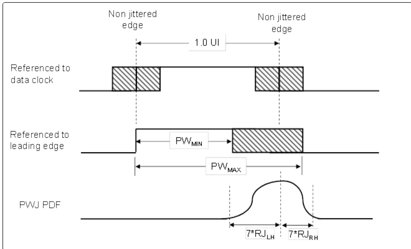
Figure 8-18 PWJ Relative to Consecutive Edges 1 UI Apart
