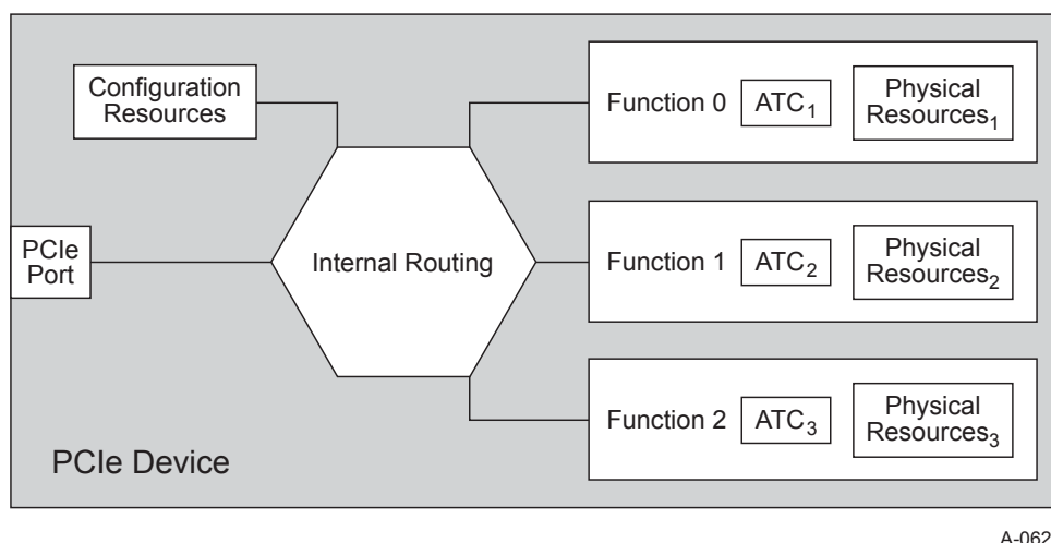
Figure 9-4 Example Multi-Function Device
